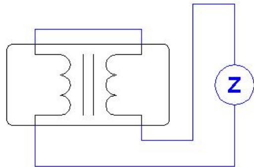
(B): Differential mode
